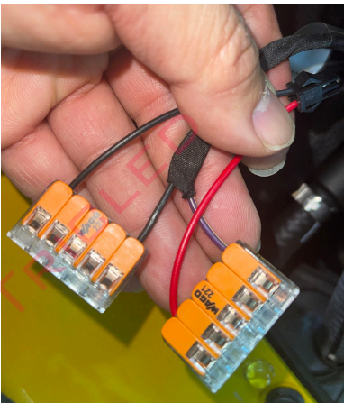
Attach the provided female connector. Black to black ground and red to positive
