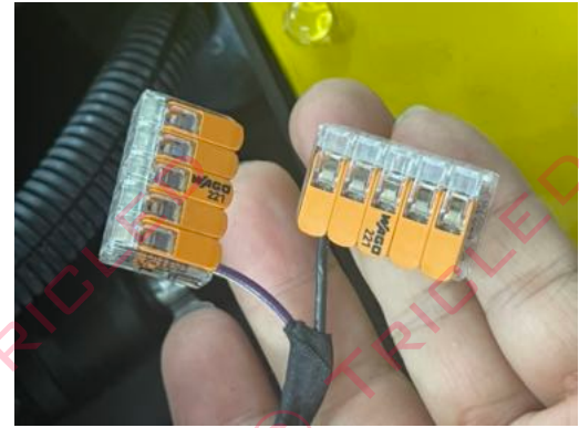
Use the lever locks, insert ground on one and positive on the other lever lock
