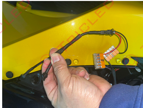
Attach the female connector to the 1:2 splitter provided. Then connect 12" extension to the left shifter side bottle LED
